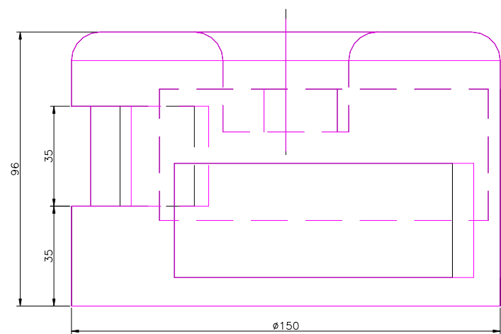
PRONT 1/2 SCALE
