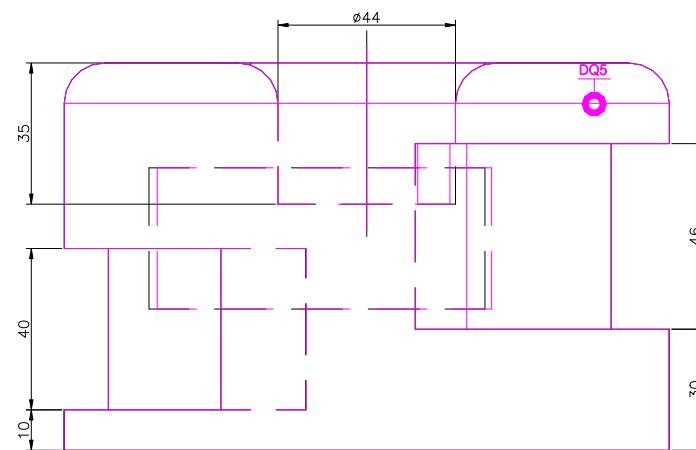
RIGHT 1/2 SCALE
