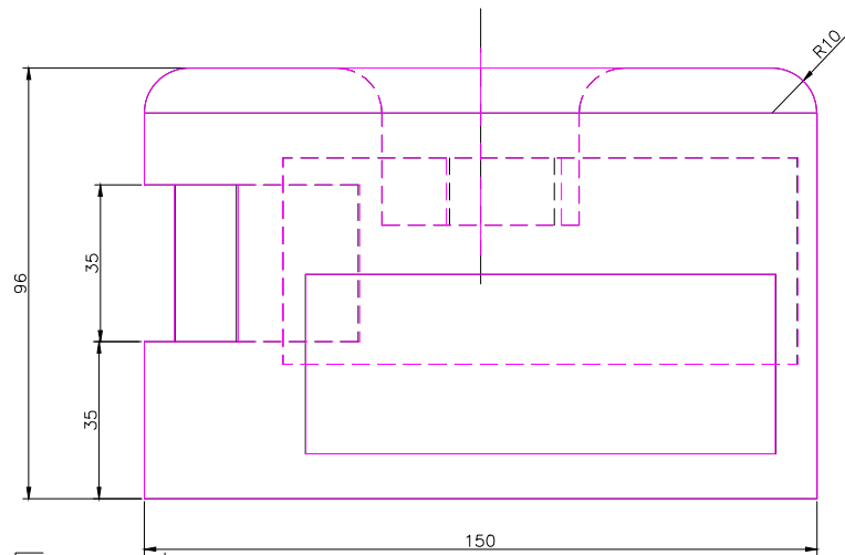
Front Scale 1/2
