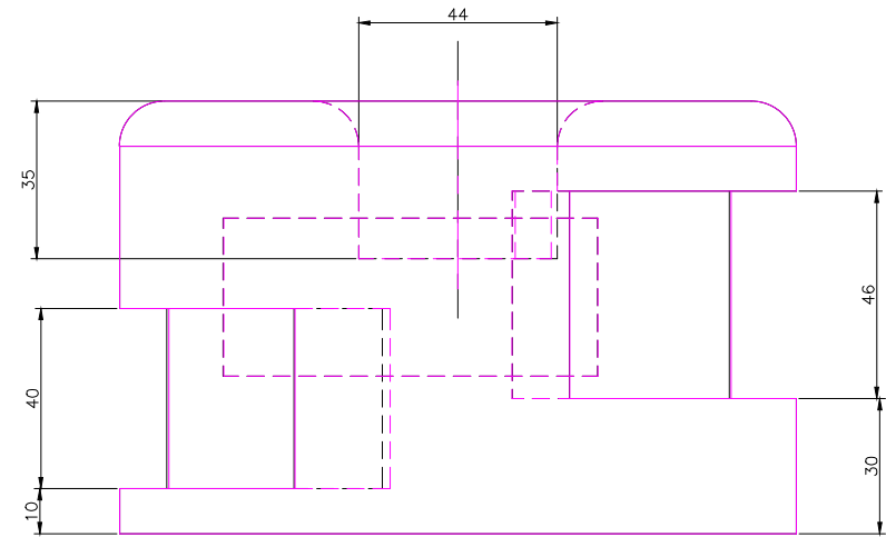
Right Scale 1/2
