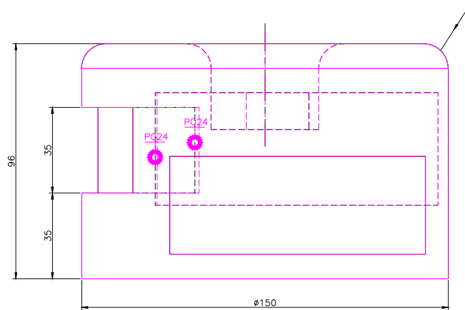
FRONT SCALE 1/2
