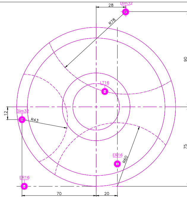
TOP SCALE 1/2
