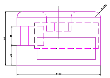
FRONT SCALE 1/2
