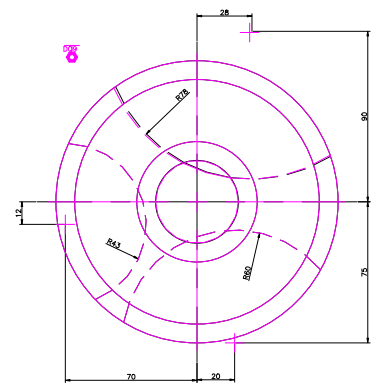
TOP SCALE 1/2
