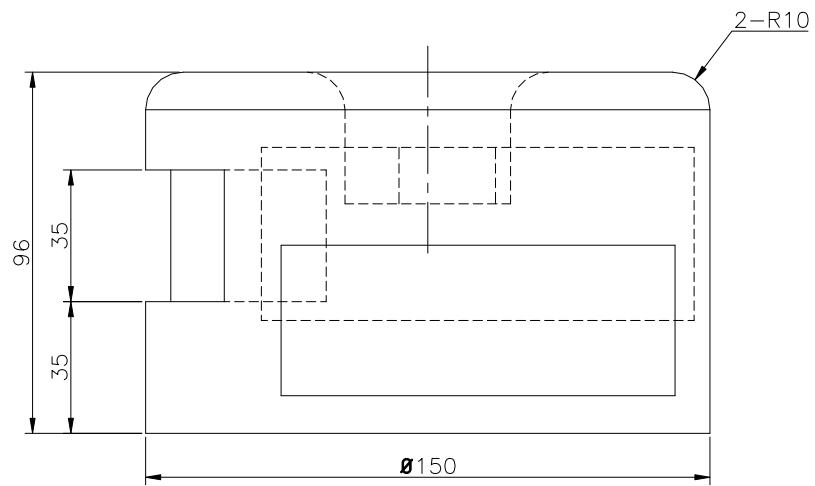
FRONT SCALE 1/2
