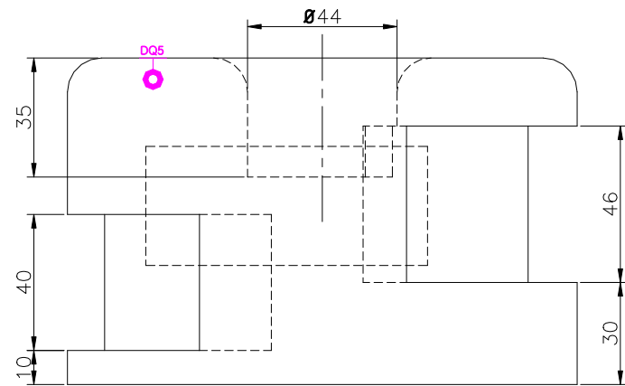
RIGHT SCALE 1/2
