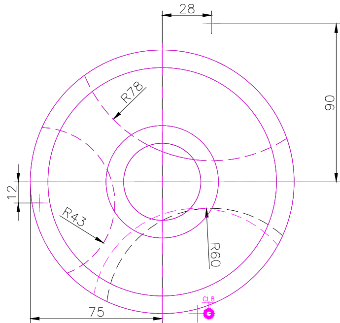
TOP SCALE 1/2
