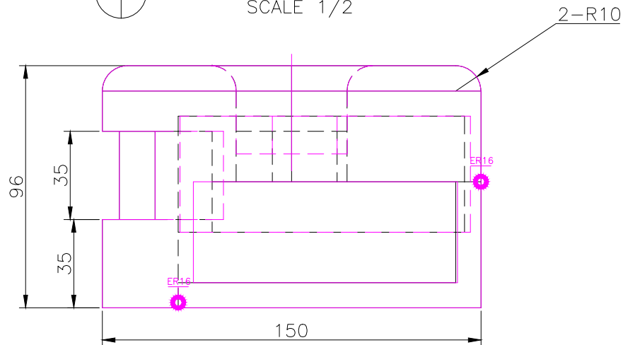
FRONT SCALE 1/2
