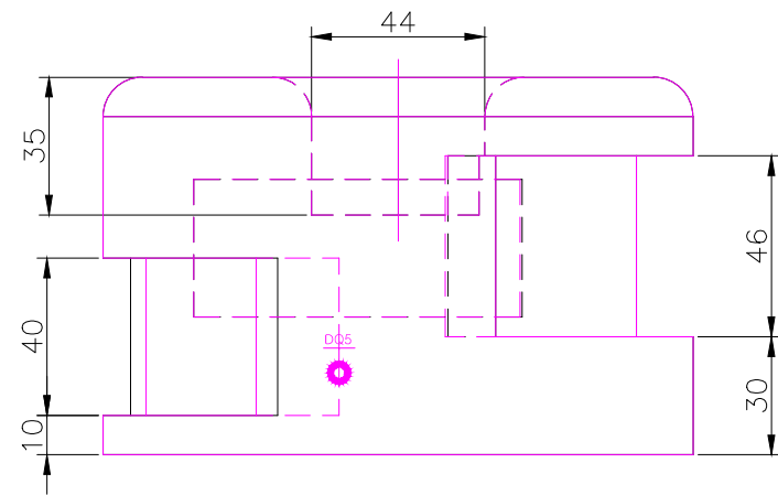
RIGHT SCALE 1/2
