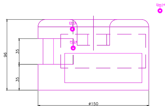
FRONT SCALE 1/2
