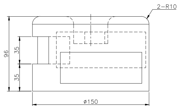
FRONT SCALE 1/2
