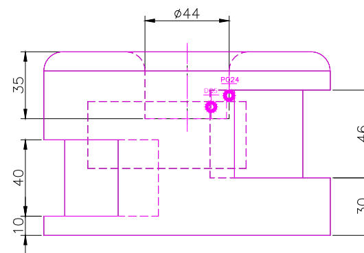
RIGHT SCALE 1/2
