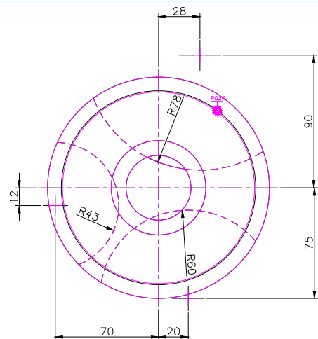
TOP SCALE 1/2
