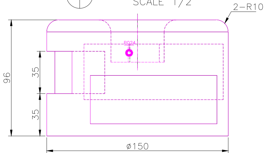
FRONT SCALE 1/2
