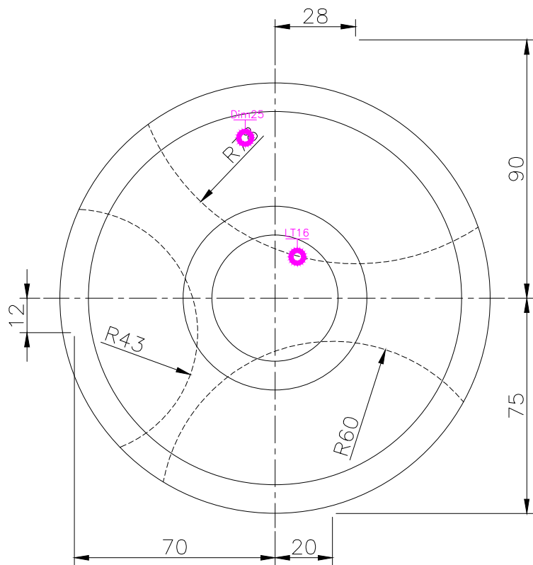
TOP SCALE 1/2
