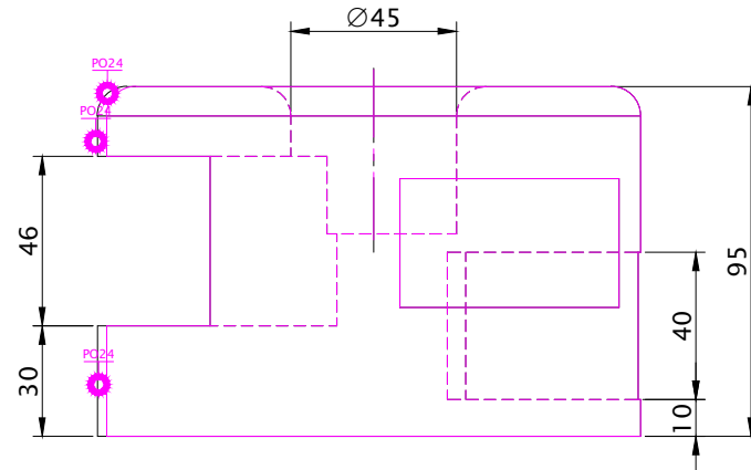
RIGHT SCALE 1/2
