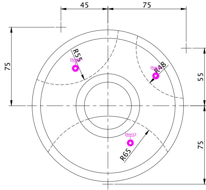
TOP SCALE 1/2
