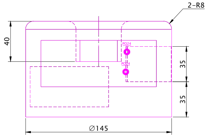
FRONT SCALE 1/2
