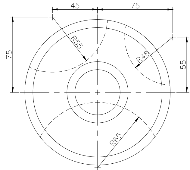
TOP SCALE 1/2
