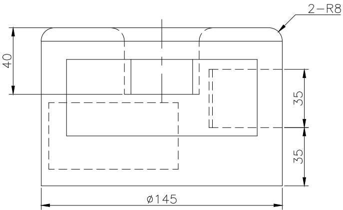
FRONT SCALE 1/2
