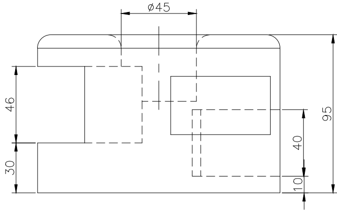
RIGHT SCALE 1/2
