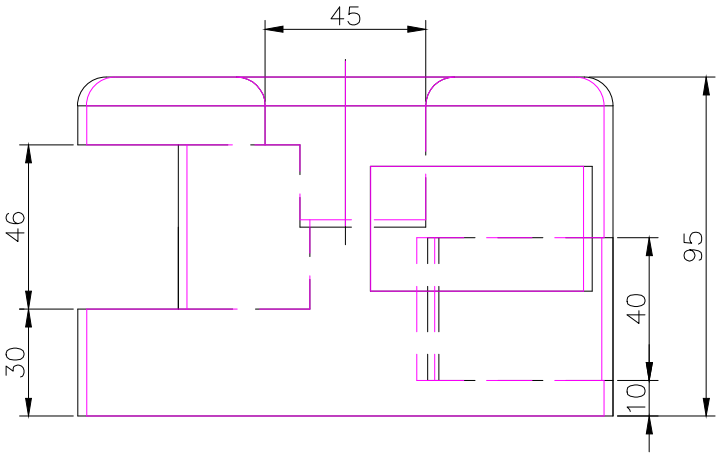
RIGHT SCALE 1/2
