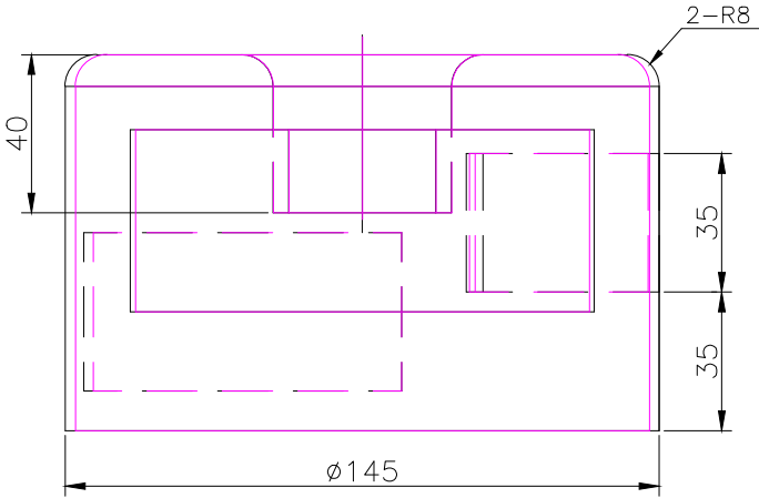
FRONT SCALE 1/2
