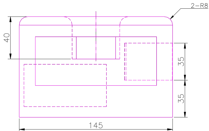
FRONT SCALE 1/2
