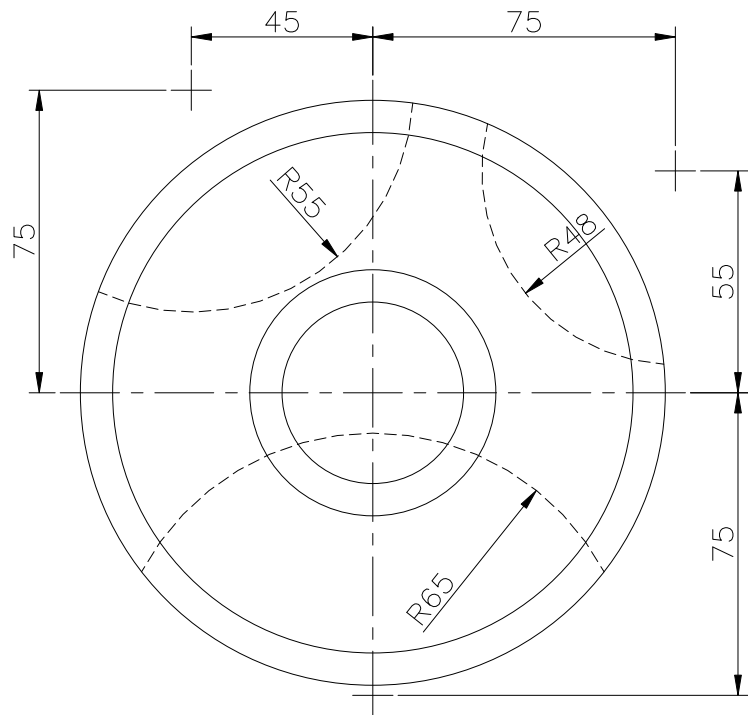
TOP SCALE 1/2
