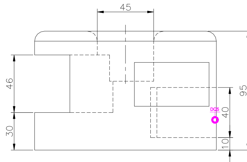
RIGHT SCALE 1/2
