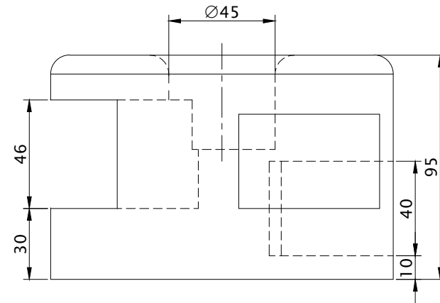
RIGHT SCALE 1/2
