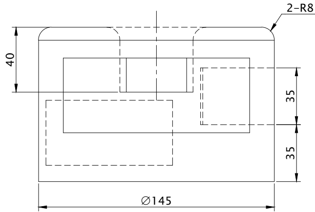
FRONT SCALE 1/2
