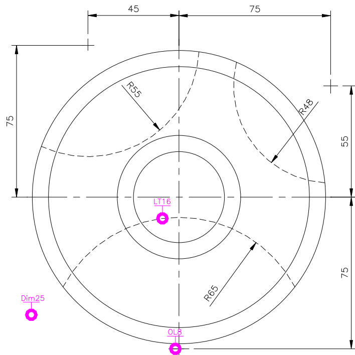
TOP SCALE 1/2
