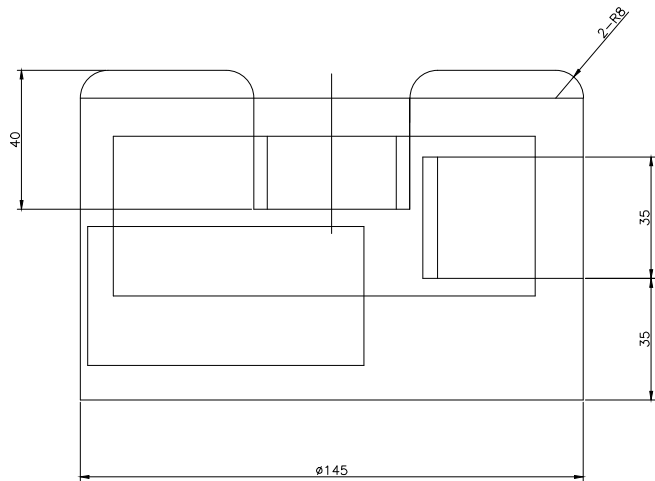
FRONT SCALE 1/2
