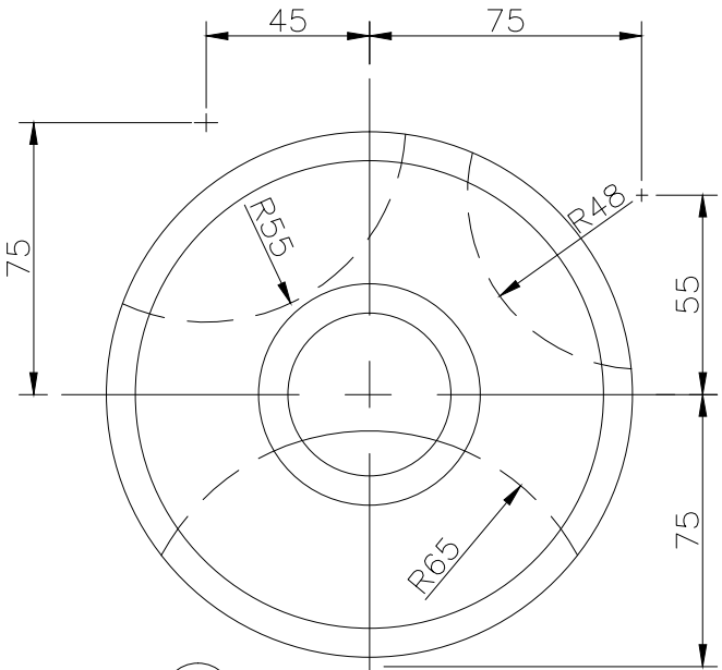
TOP SCALE 1/2
