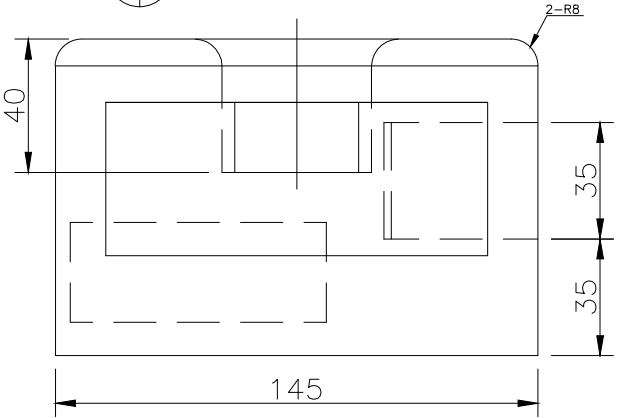
FRONT SCALE 1/2
