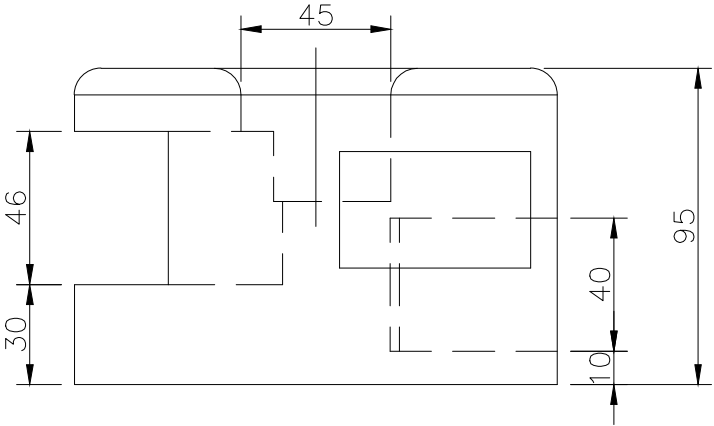
RIGHT SCALE 1/2
