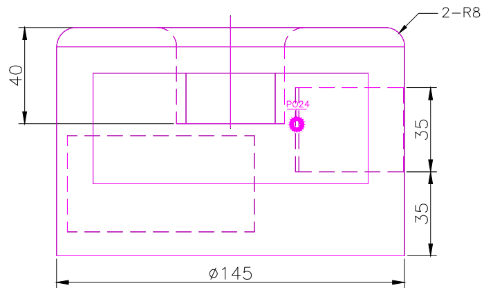
FRONT SCALE 1/2
