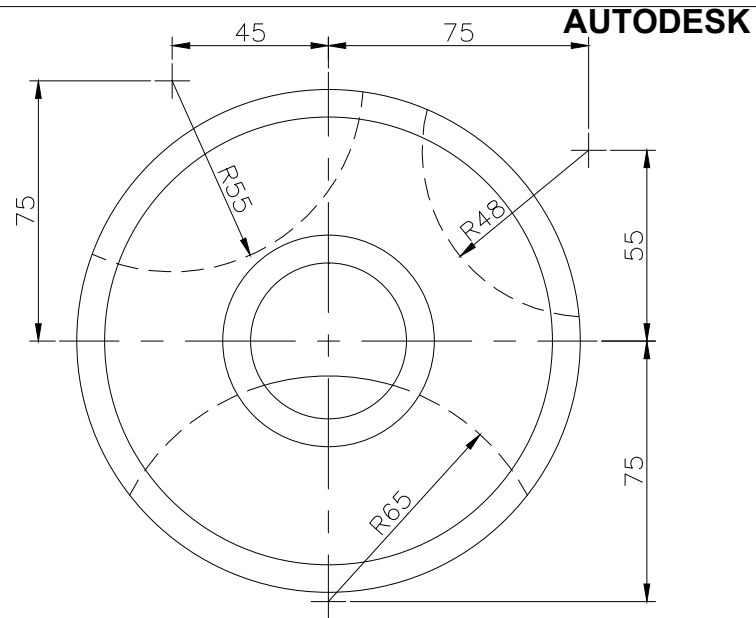
TOP SCALE 1/2
