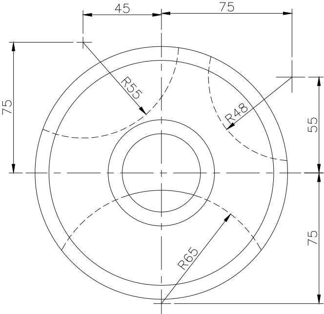
TOP SCALE 1/2
