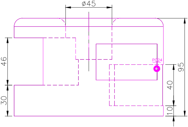
RIGHT SCALE 1/2
