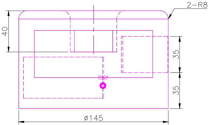
FRONT SCALE 1/2
