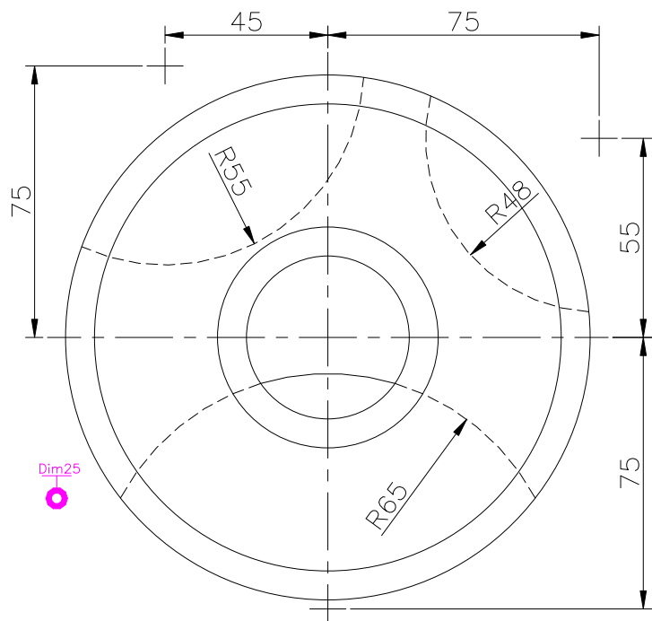
TOP SCALE 1/2
