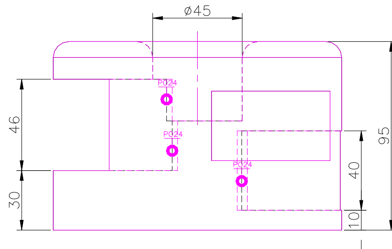
RIGHT SCALE 1/2
