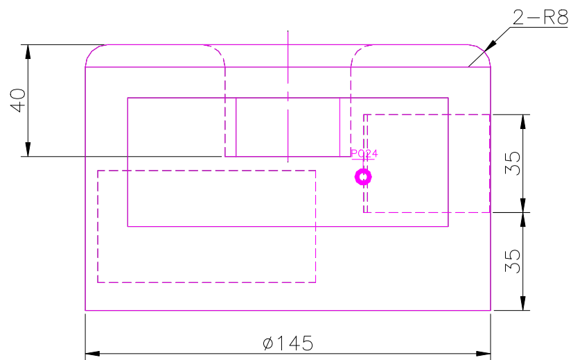
FRONT SCALE 1/2
