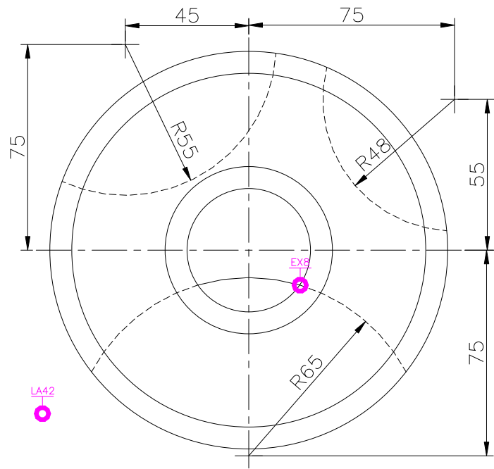
TOP SCALE 1/2
