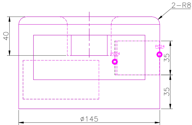
FRONT SCALE 1/2
