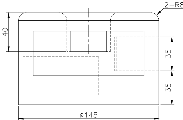
FRONT SCALE 1/2
