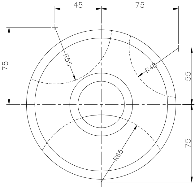
TOP SCALE 1/2
