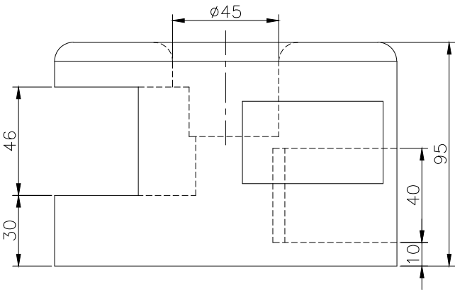
RIGHT SCALE 1/2
