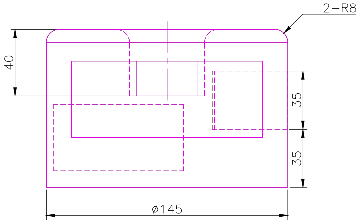
FRONT SCALE 1/2
