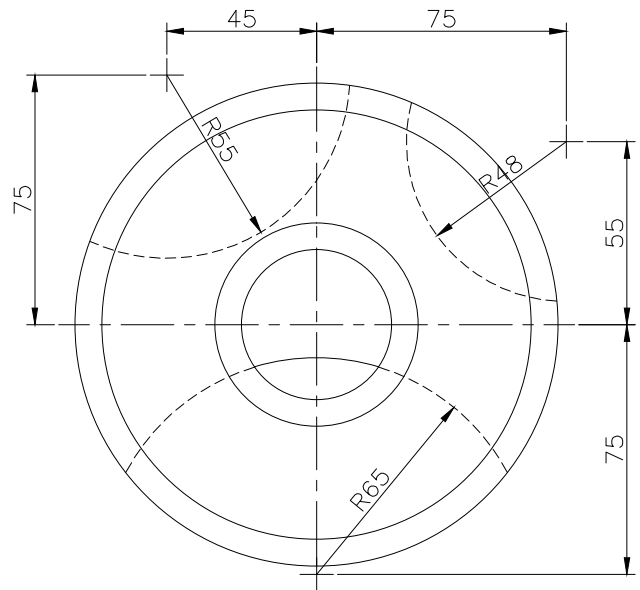
TOP SCALE 1/2
