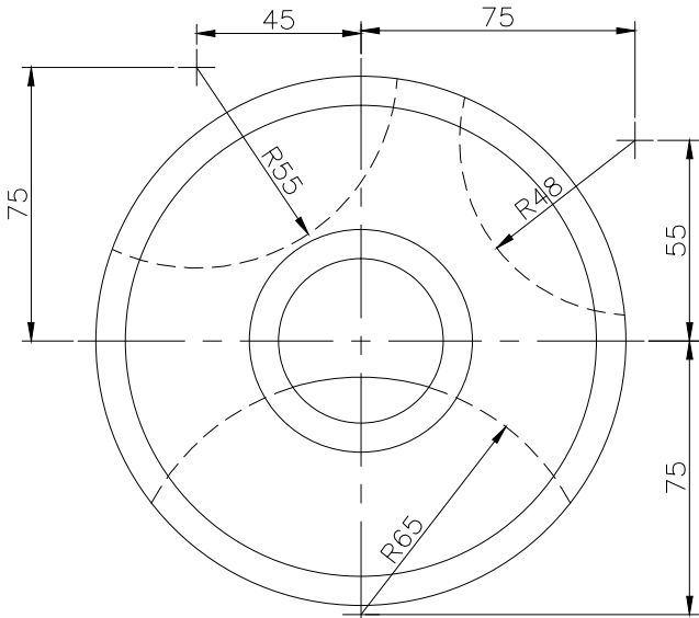
TOP SCALE 1/2
