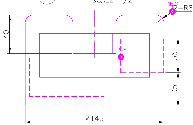
FRONT SCALE 1/2
