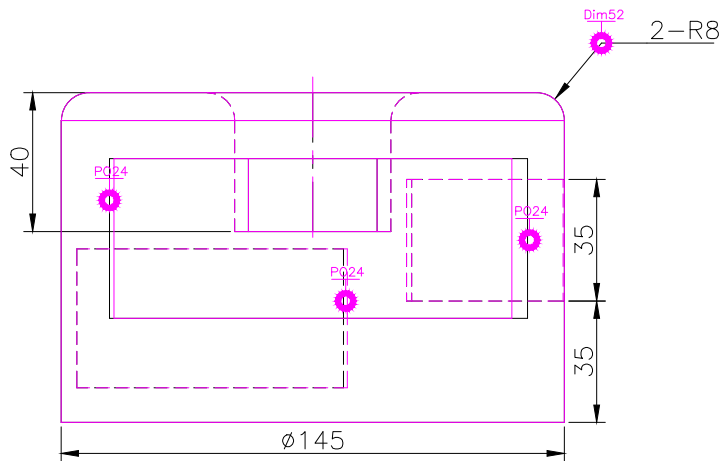
FRONT SCALE 1/2
