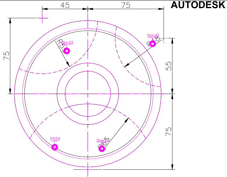
TOP SCALE 1/2
