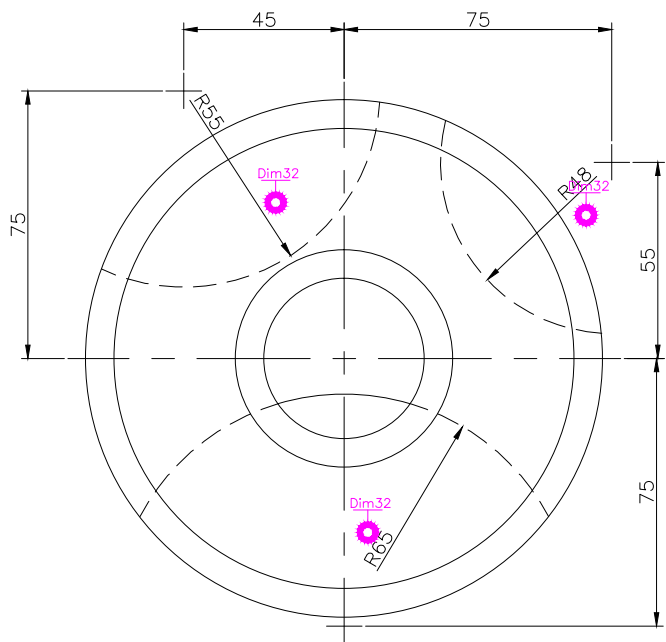
TOP SCALE 1/2
