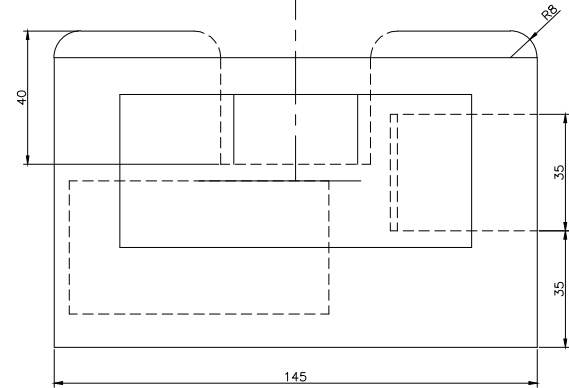
FRONT SCALE 1/2
