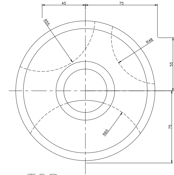
TOP SCALE 1/2
