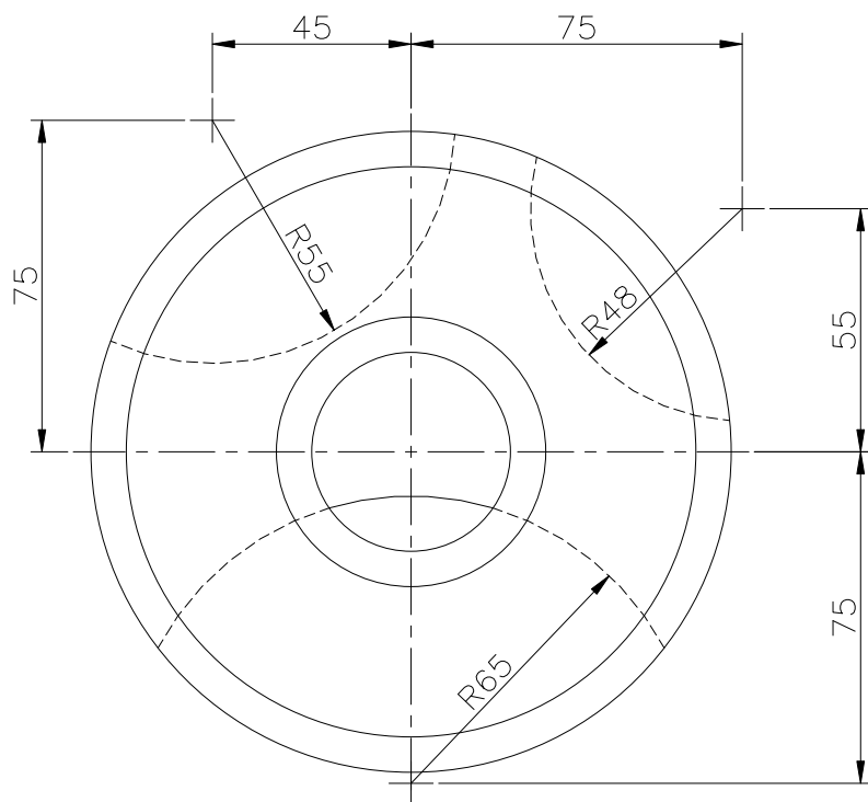
TOP SCALE 1/2
