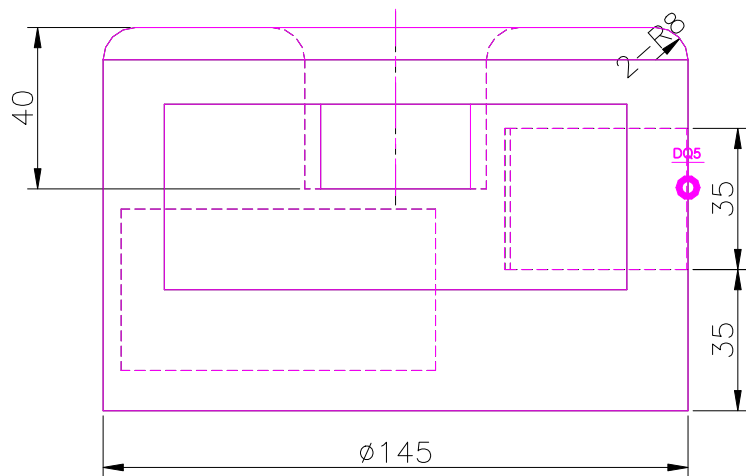
FRONT SCALE 1/2
