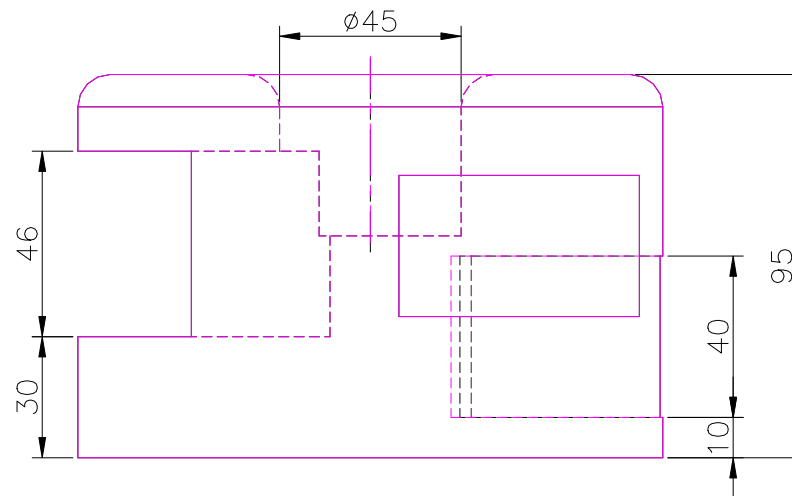
RIGHT SCALE 1/2
