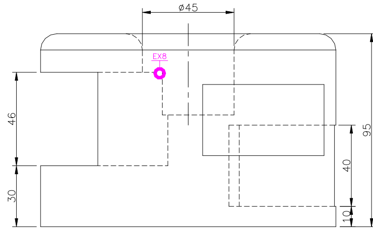
RIGHT SCALE 1/2
