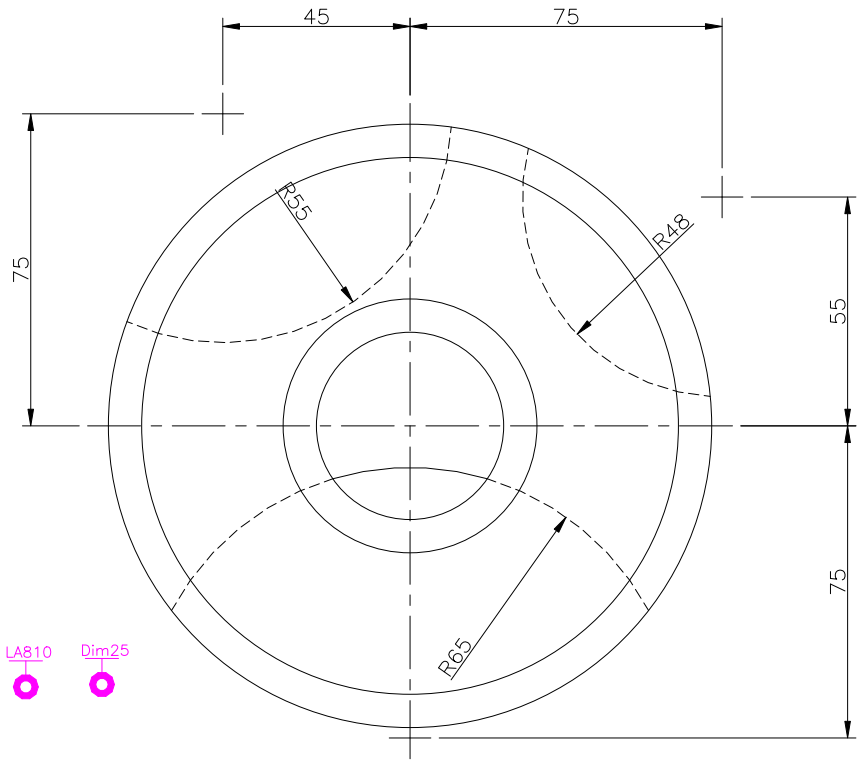
TOP SCALE 1/2
