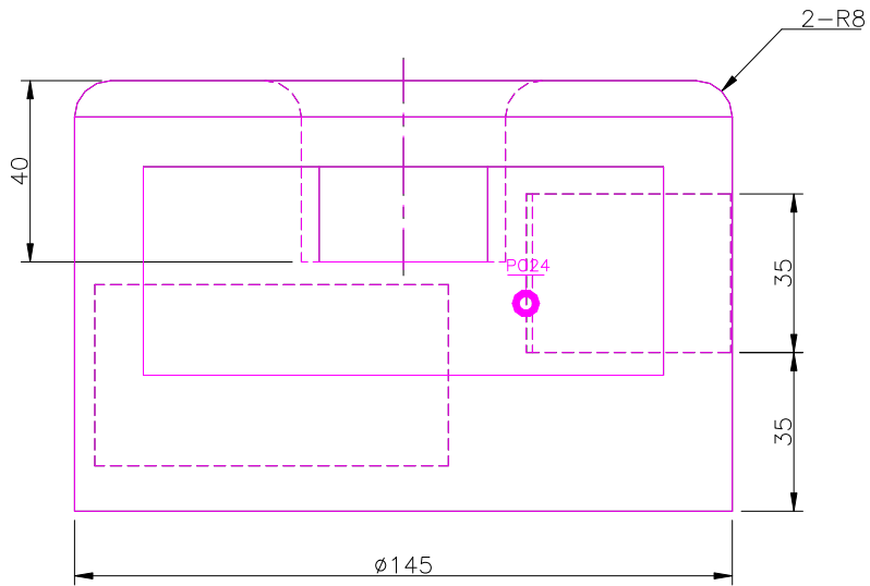
FRONT SCALE 1/2
