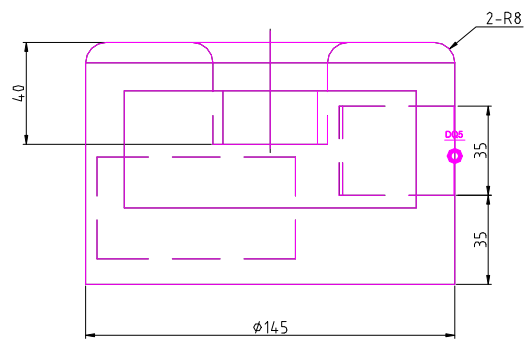
FRONT SCALE 1/2
