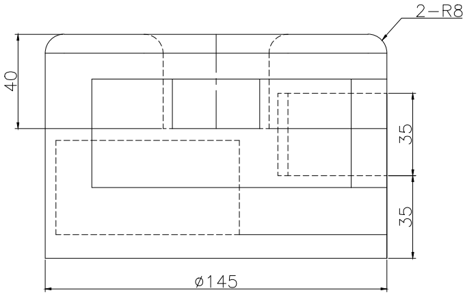
FRONT SCALE 1/2
