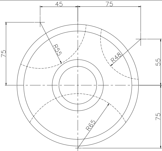
TOP SCALE 1/2
