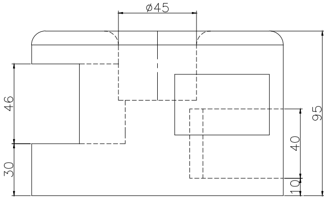
RIGHT SCALE 1/2
