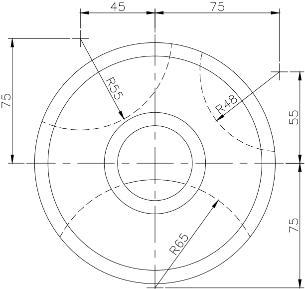
TOP SCALE 1/2
