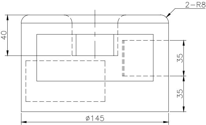
FRONT SCALE 1/2
