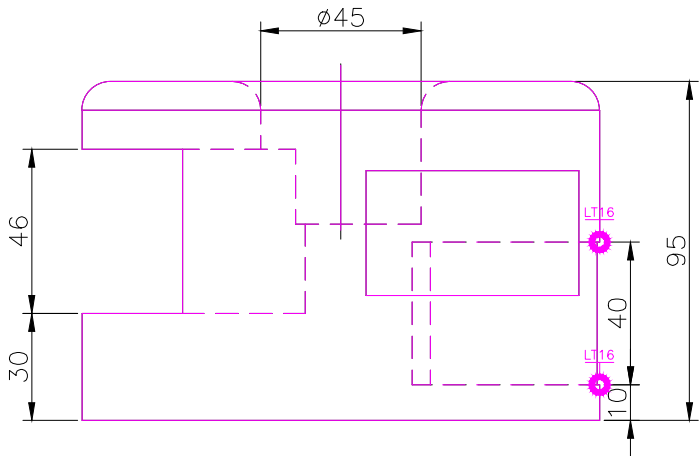
RIGHT SCALE 1/2
