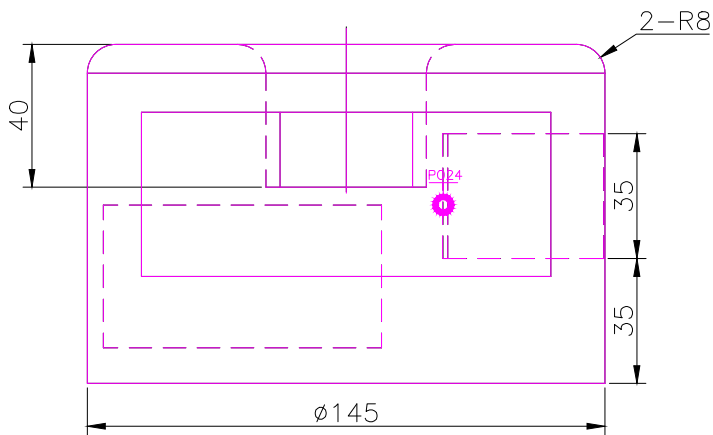
FRONT SCALE 1/2
