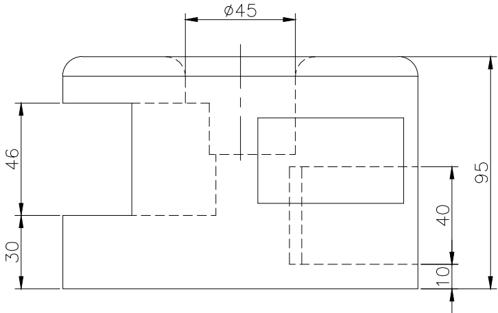
RIGHT SCALE 1/2
