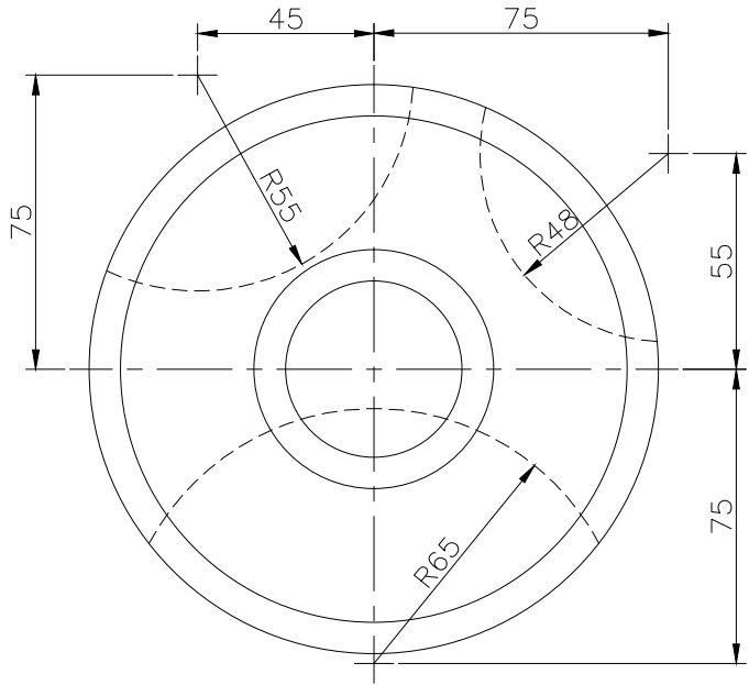
TOP SCALE 1/2
