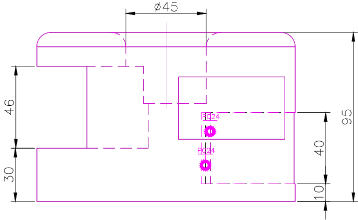
RIGHT SCALE 1/2
