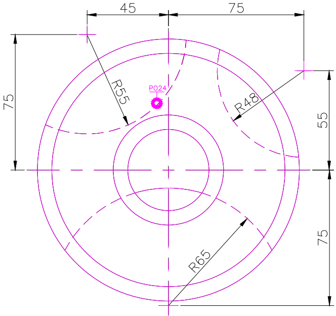
TOP SCALE 1/2
