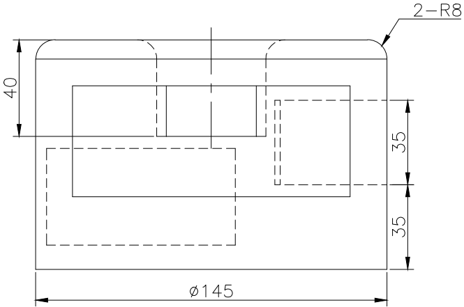
FRONT SCALE 1/2
