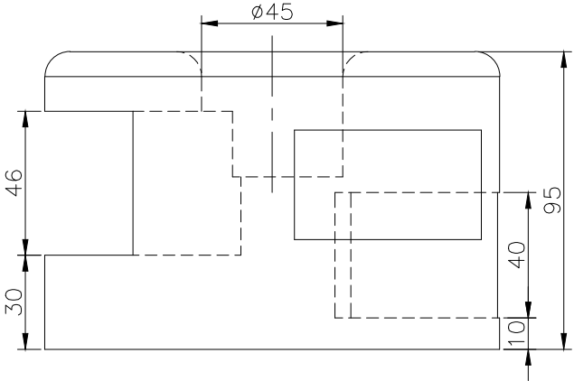
RIGHT SCALE 1/2
