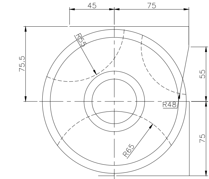
TOP SCALE 1/2
