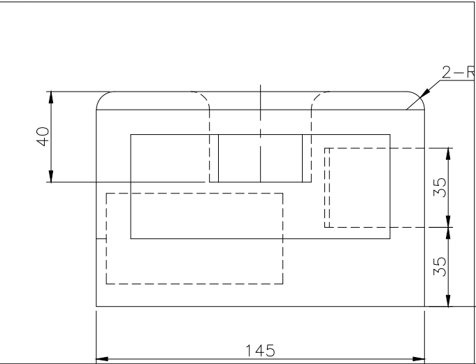
FRONT SCALE 1/2
