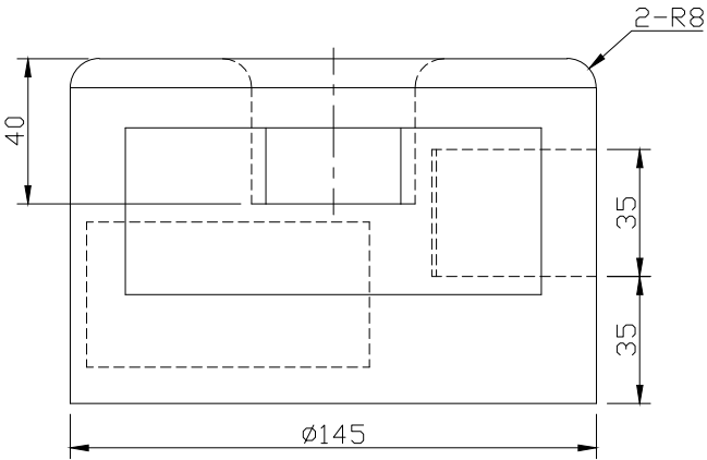
FRONT SCALE 1/2
