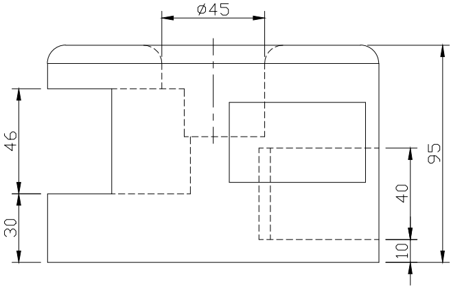
RIGHT SCALE 1/2
