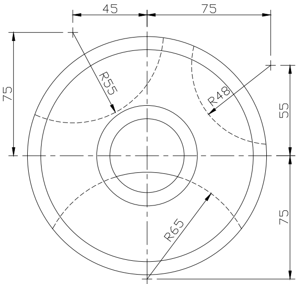
TOP SCALE 1/2
