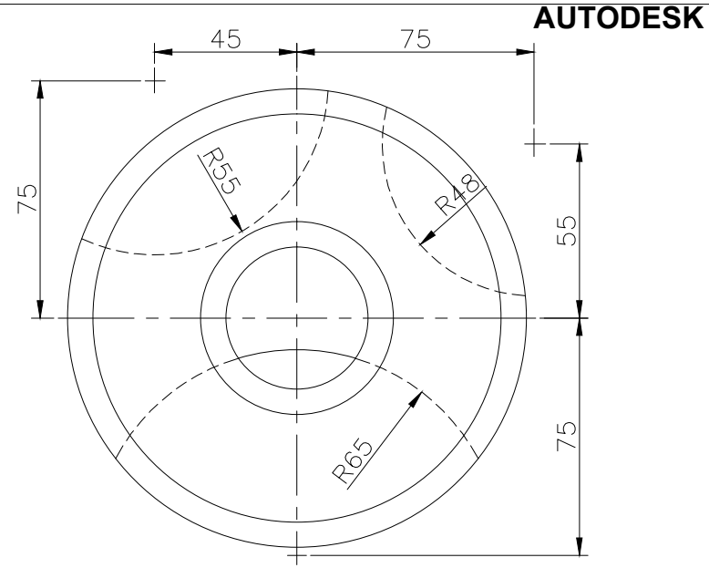
TOP SCALE 1/2
