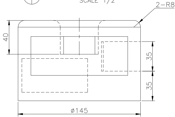
FRONT SCALE 1/2
