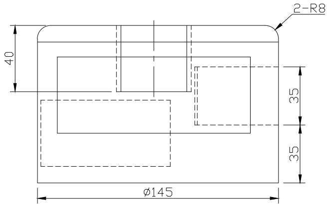
FRONT SCALE 1/2
