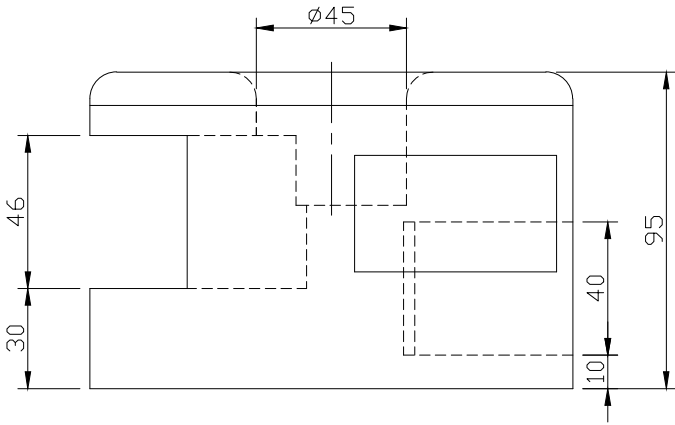
RIGHT SCALE 1/2
