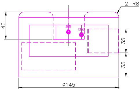
FRONT SCALE 1/2
