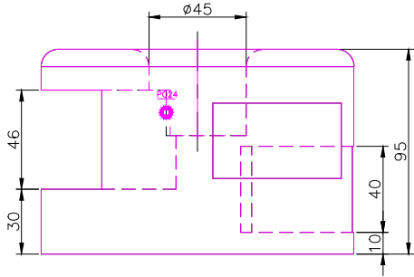
RIGHT SCALE 1/2
