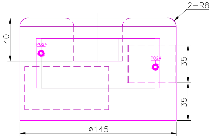
FRONT SCALE 1/2
