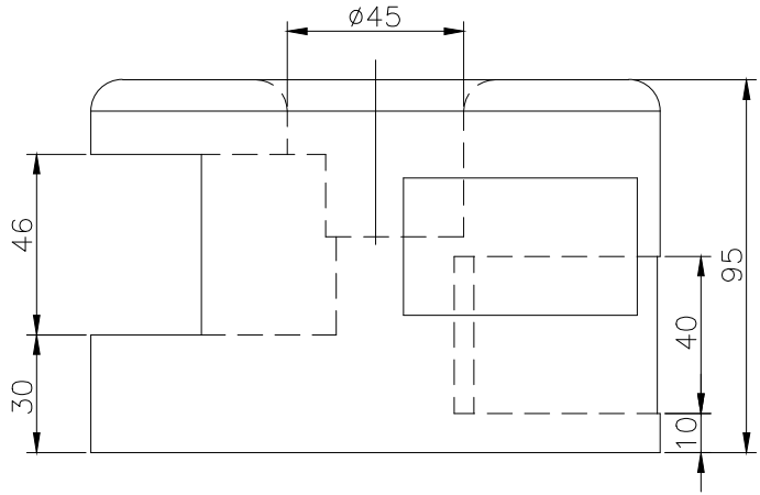
RIGHT SCALE 1/2
