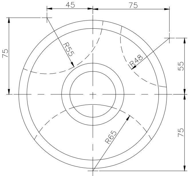
TOP SCALE 1/2
