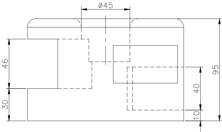
RIGHT SCALE 1/2
