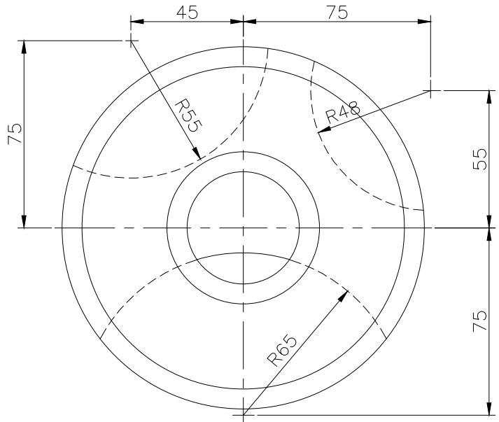
TOP SCALE 1/2
