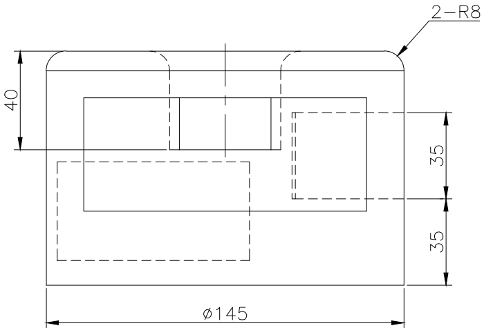
FRONT SCALE 1/2
