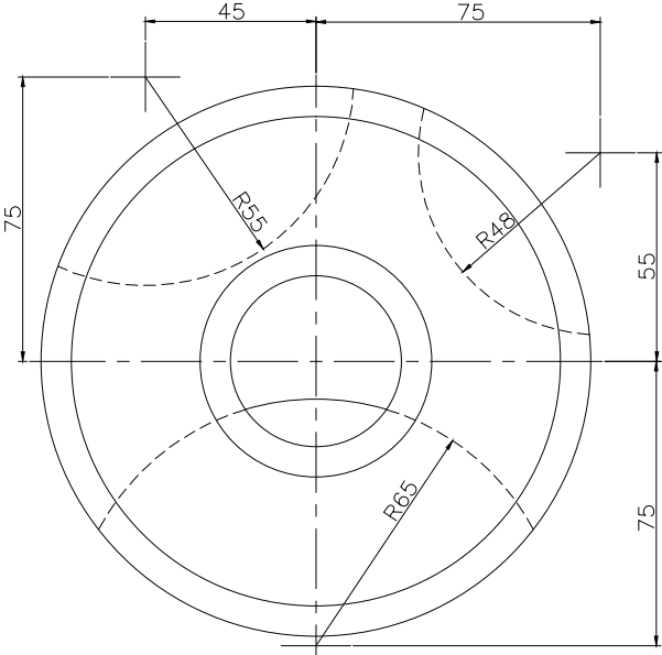
TOP SCALE 1/2
