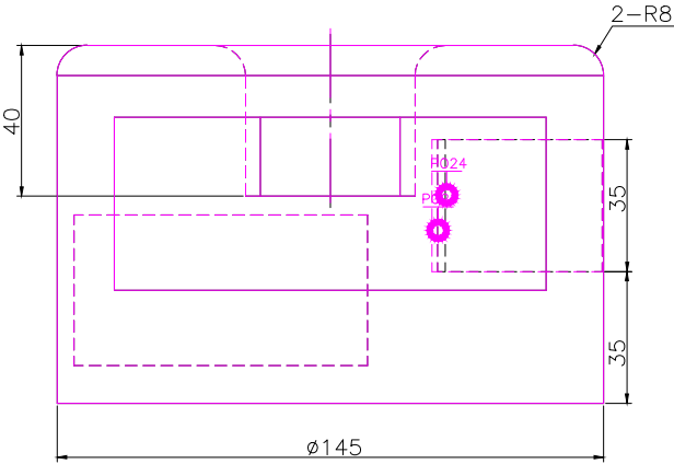
FRONT SCALE 1/2
