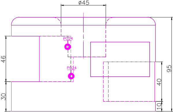
RIGHT SCALE 1/2
