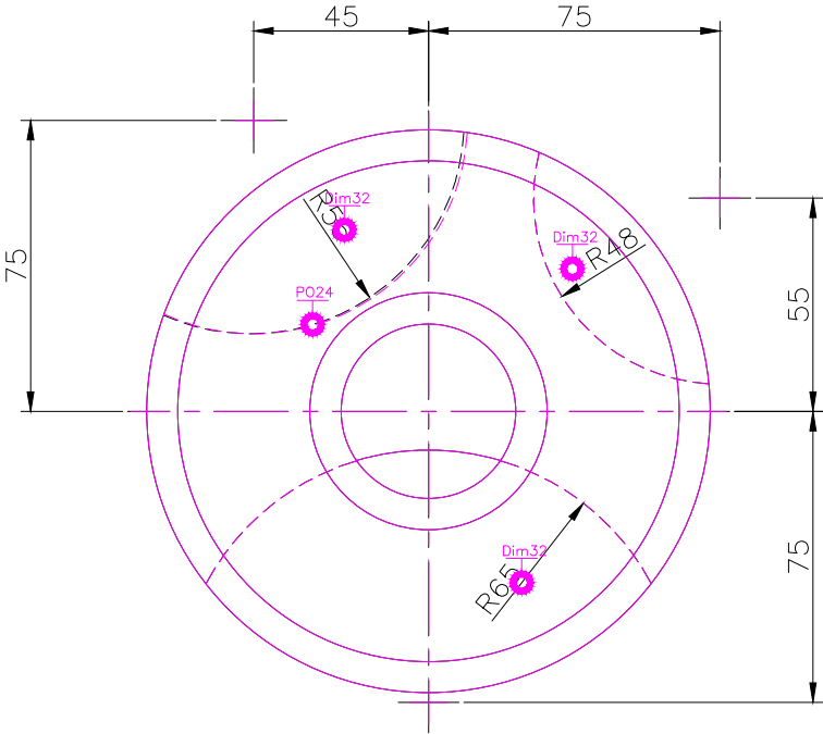
TOP SCALE 1/2
