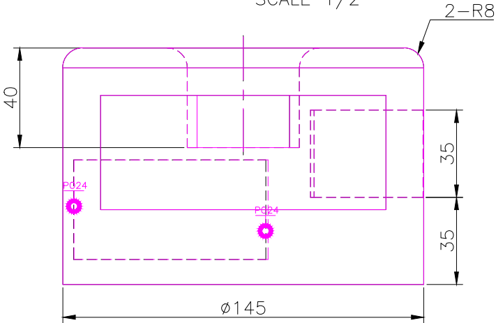
FRONT SCALE 1/2
