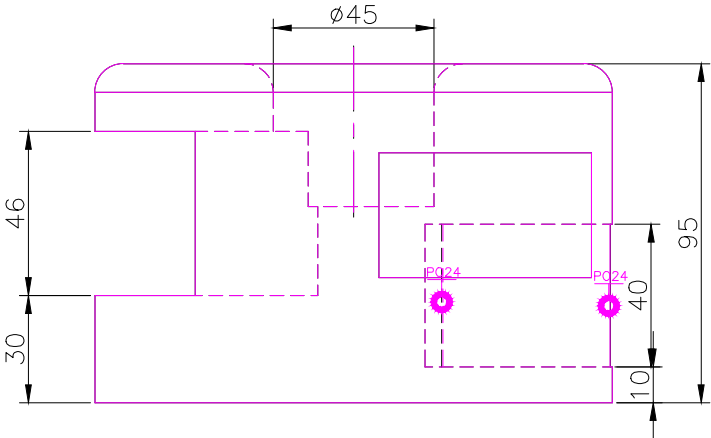
RIGHT SCALE 1/2
