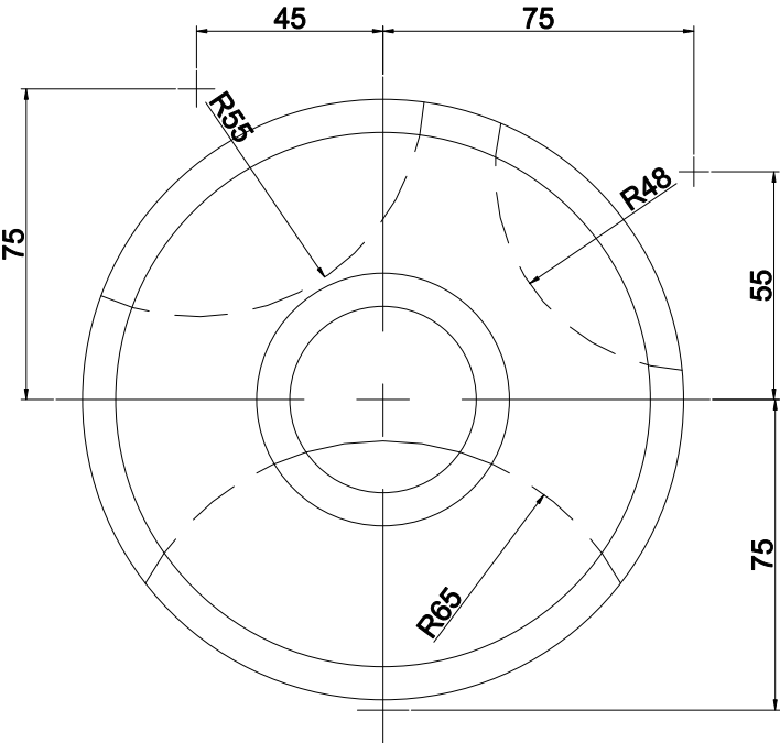
TOP SCALE 1/2
