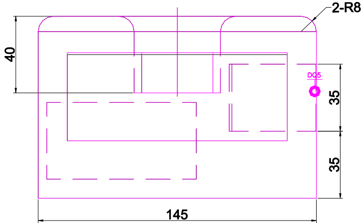
FRONT SCALE 1/2
