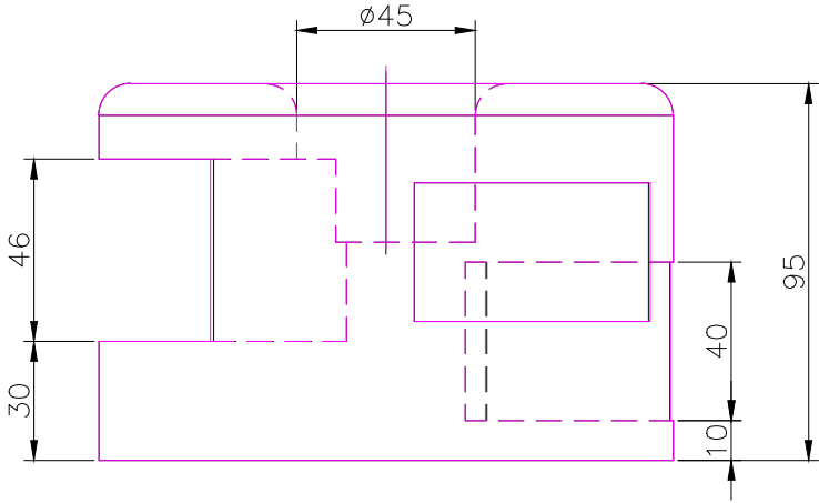
RIGHT SCALE 1/2
