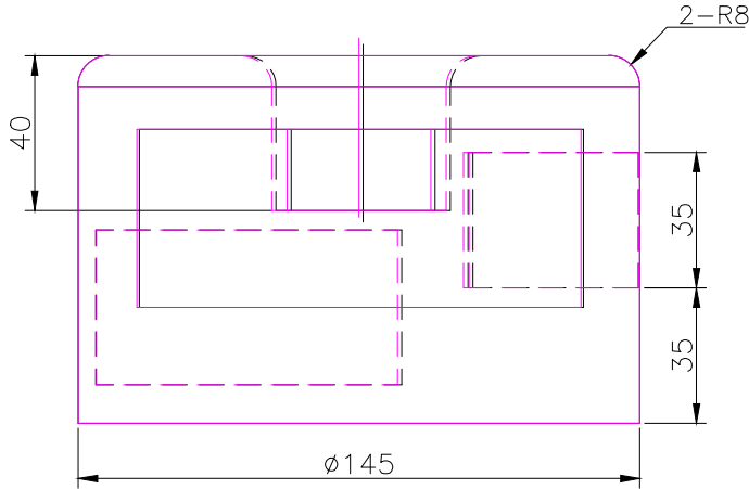
FRONT SCALE 1/2
