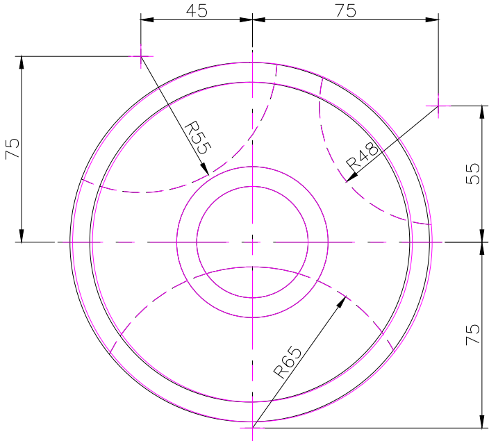
TOP SCALE 1/2
