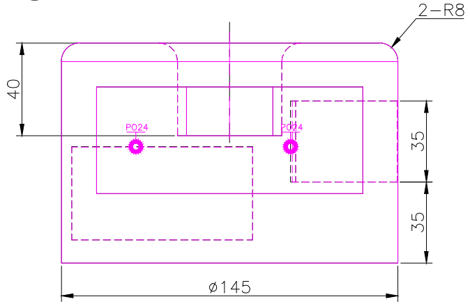
FRONT SCALE 1/2
