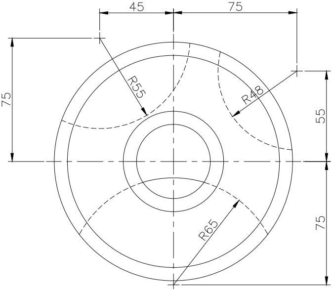
TOP SCALE 1/2
