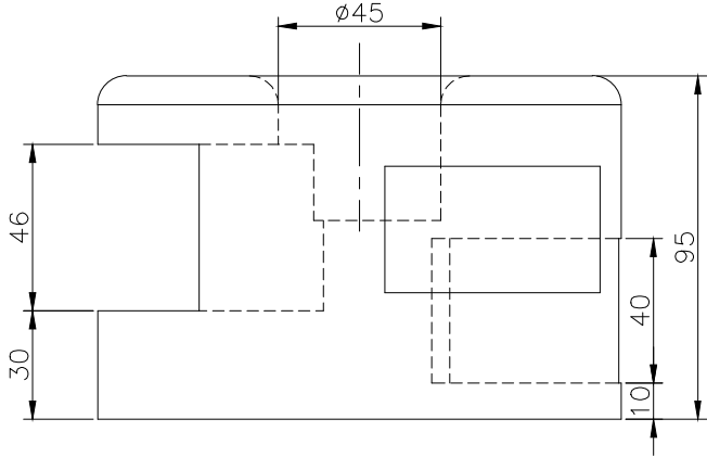
RIGHT SCALE 1/2
