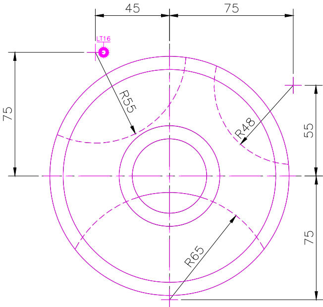
TOP SCALE 1/2
