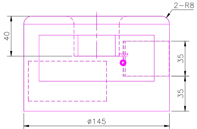
FRONT SCALE 1/2
