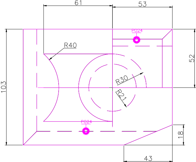
TOP SCALE 1/2
