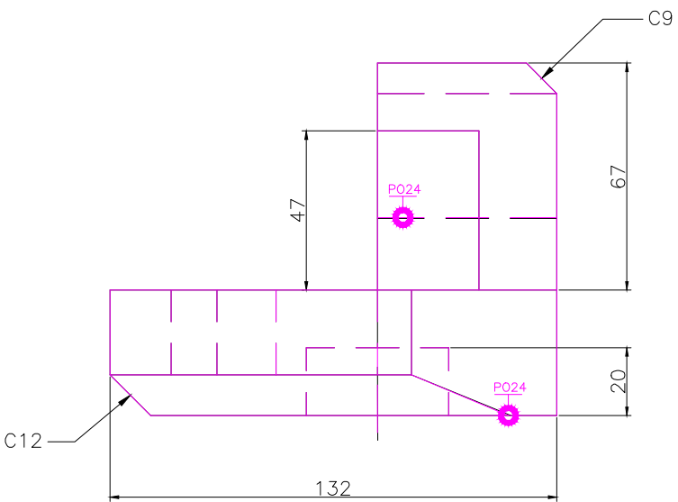
FRONT SCALE 1/2
